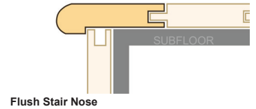
Flush Stair Nose
