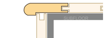
Flush Stair Nose
